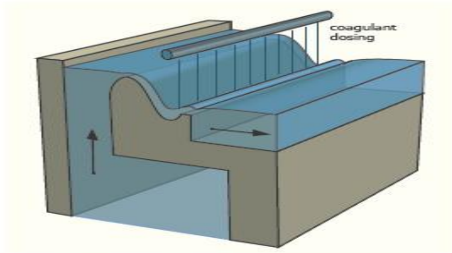
Figure 17 - Cascade mixer
