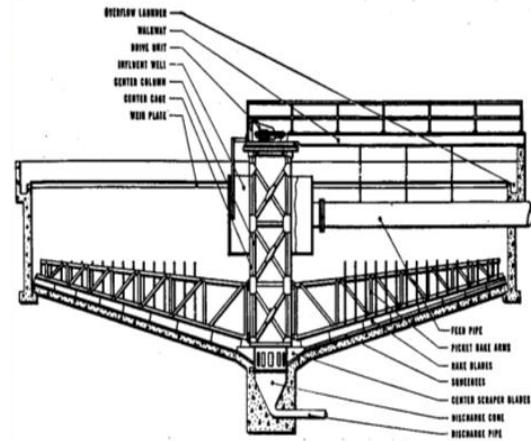
Fig. 5-19 Continuous flow thickeners.
