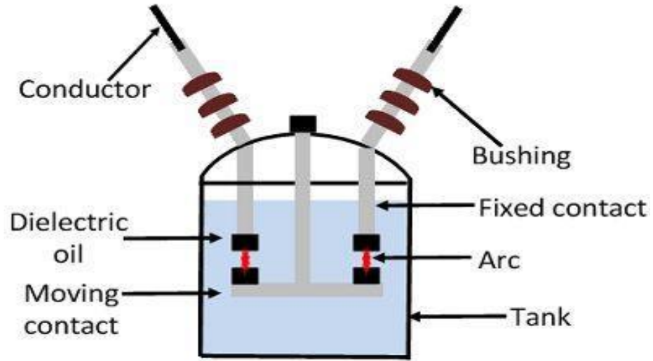
Bulk Oil Circuit Breaker
