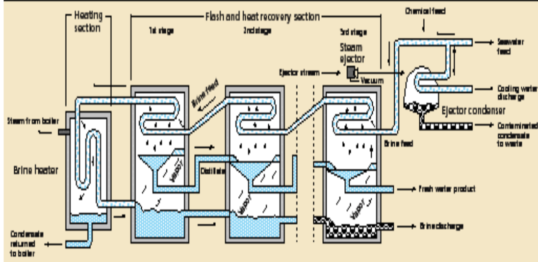
Diagram of a multistage flash distillation plant
