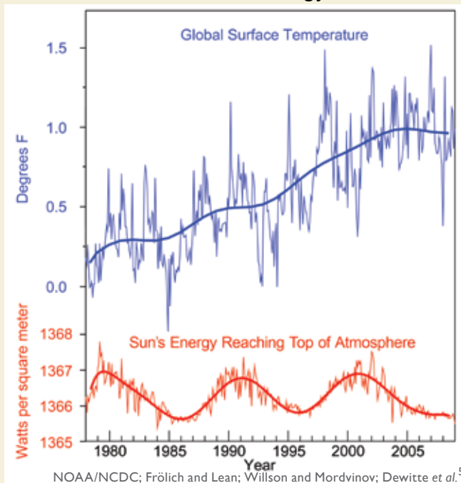
The Sun's energy received at the top of Earth's atmosphere has been measured by satellites since 1978. It has followed its natural 11-year cycle of small ups and downs, but with no net increase (bottom). Over the same period, global temperature has risen markedly (top). 60
