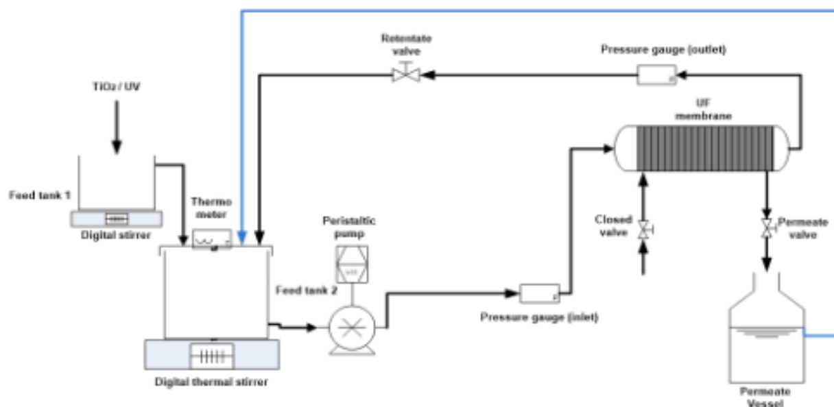
Fig. 1. Advanced Oxidation Processes (AOP) and Membrane Filtration (MF) used in an integrated wastewater treatment system. Source [13].
