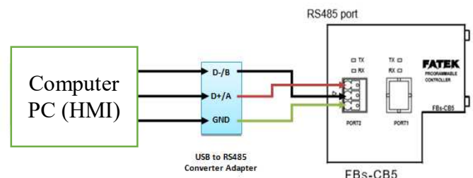
Fig. 8 Block diagram of PLC data communication to PC
