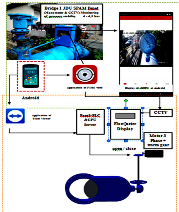
Fig. 3 Process flow of automatic valve design
