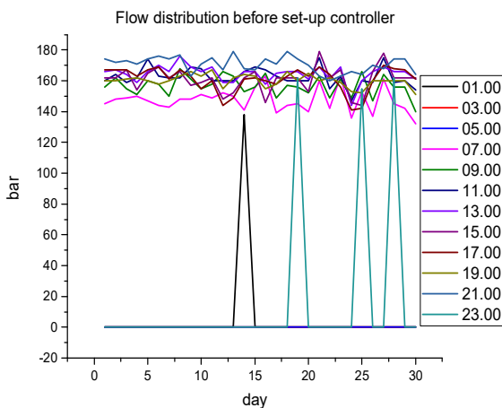
Fig. 11 Flow comparison chart before control system installation
