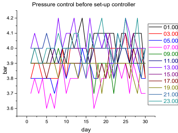
Fig. 9 Pressure comparison graph before installing the control system
