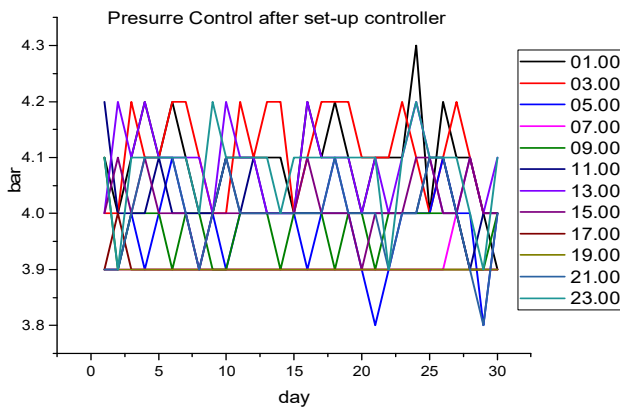
Fig. 10 Pressure comparison graph after installing the control system
