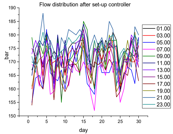
Fig. 12 Flow comparison chart after control system installation
