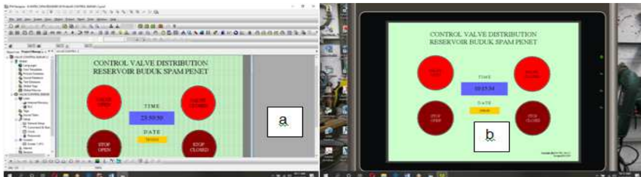
Fig. 7 Display Application for Making Ladder Diagrams (a) and Display Human Machine Interface (HMI) when running (b)
